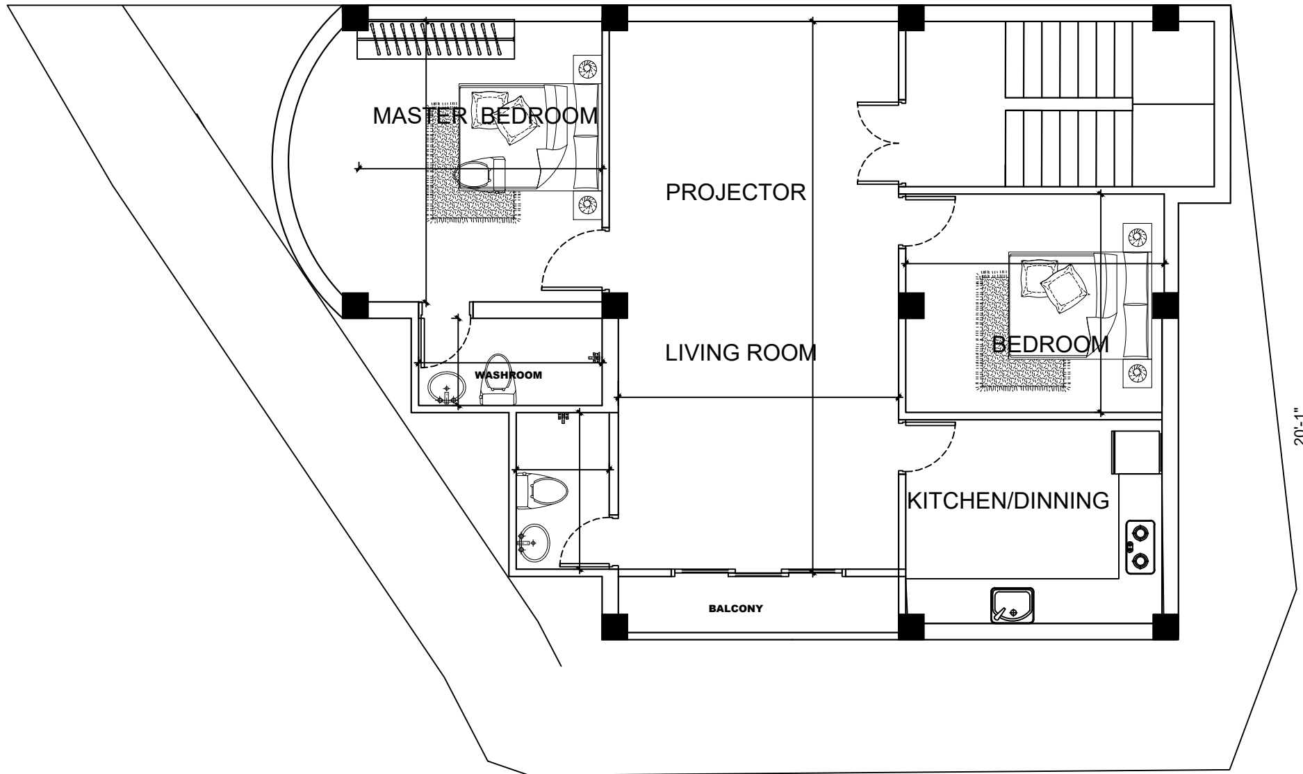
FIRST FLOOR PLAN AREA: 1060 SQ. FT
